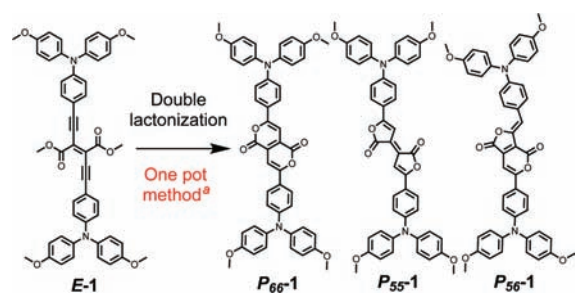
Scheme 1. Double Lactonization in E -1 and the Three Resultant Triarylamine-Appended Pechmann Dyes
